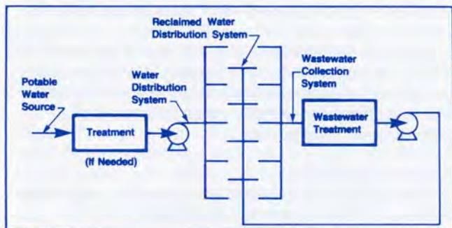
Figure 1. Dual Distribution System Schematic
