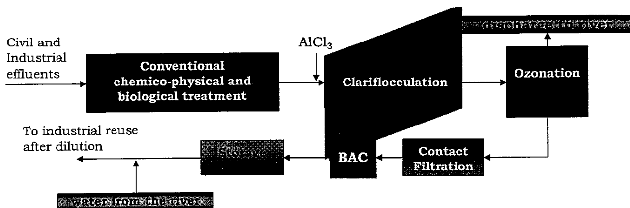
Figure 3 - Scheme of the Prato MWWTP and of the industrial refining treatment plant.
