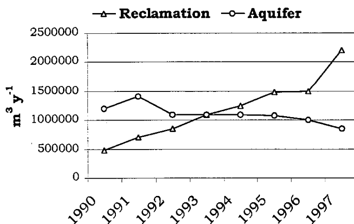
Figure 4 – Trend of the Industrial water consumption in the Prato area.
